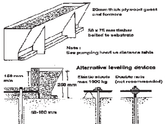
Figure 2 - Typical hopper system
